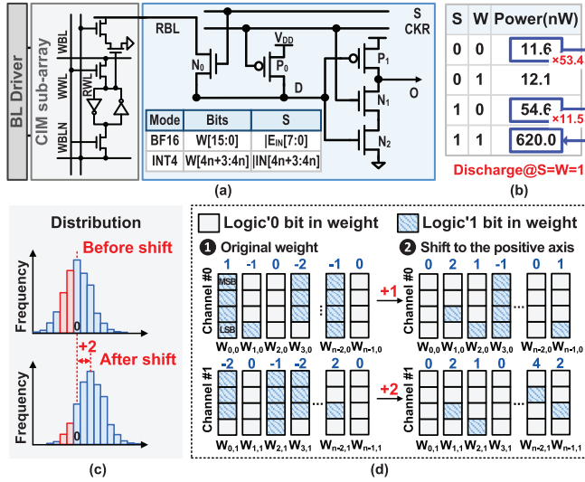
Fig. 11. (a) Sparsity-aware readout circuit. (b) Power consumption table for different readout cases, evaluated at 0.8 V, 25 °C, and 130 MHz, based on one CIM column with 16 cells. (c) Gaussian-like distribution of LLM weights. (d) Illustration of the DOWE scheme.
