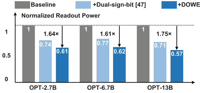
Fig. 13. Evaluation for the readout power under different weight-sparse encoding schemes on multiple OPT family models. Baseline: pre-trained model under ONAQ. “+Dual-sign-bit”: optimize the baseline with dual-sign-bit encoding scheme in [47]. “+DOWE”: optimize the baseline with DOWE.
