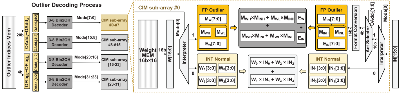
Fig. 5. Outlier-normal decoding process and mode configuration.
