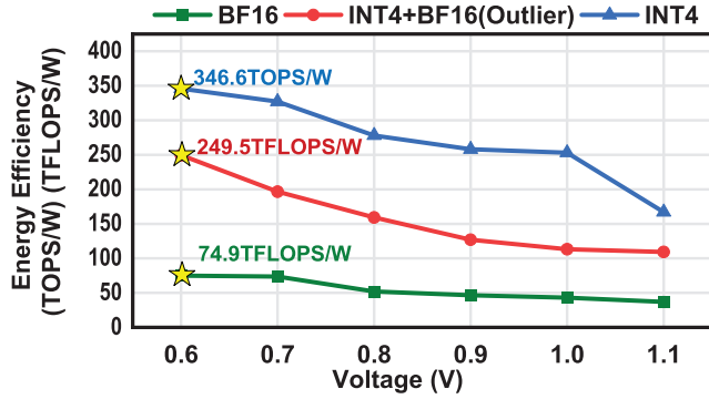
Fig. 17. Measured voltage-EEF scaling.
