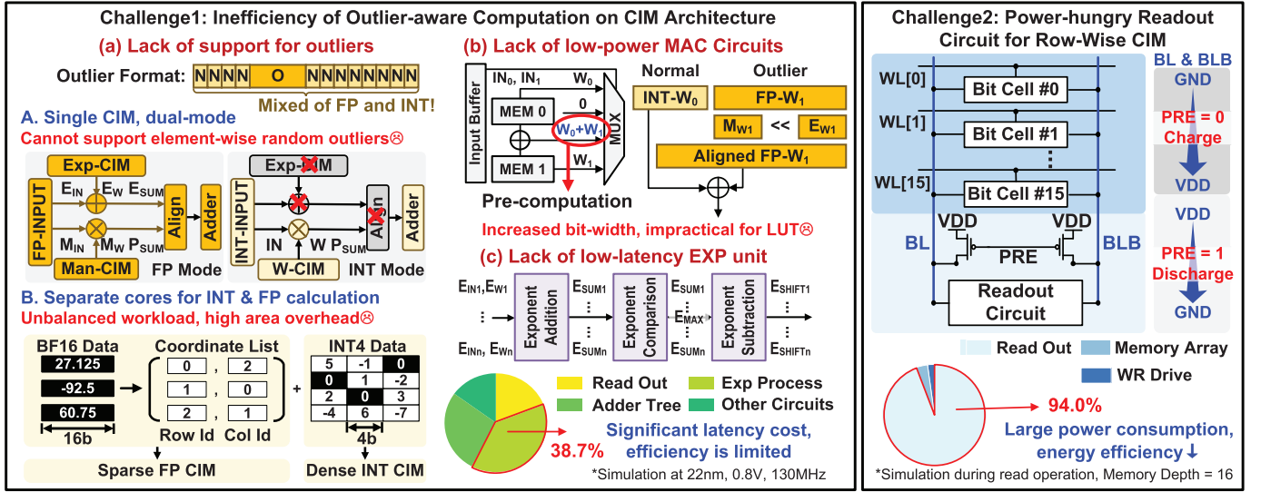
Fig. 2. Key challenges in designing a CIM processor for LLM acceleration: Inefficient handling of outliers and high-power readout operations. (a) Lack of support for outliers. (b) Lack of low-power MAC Circuits. (c) Lack of a low-latency EXP unit.
