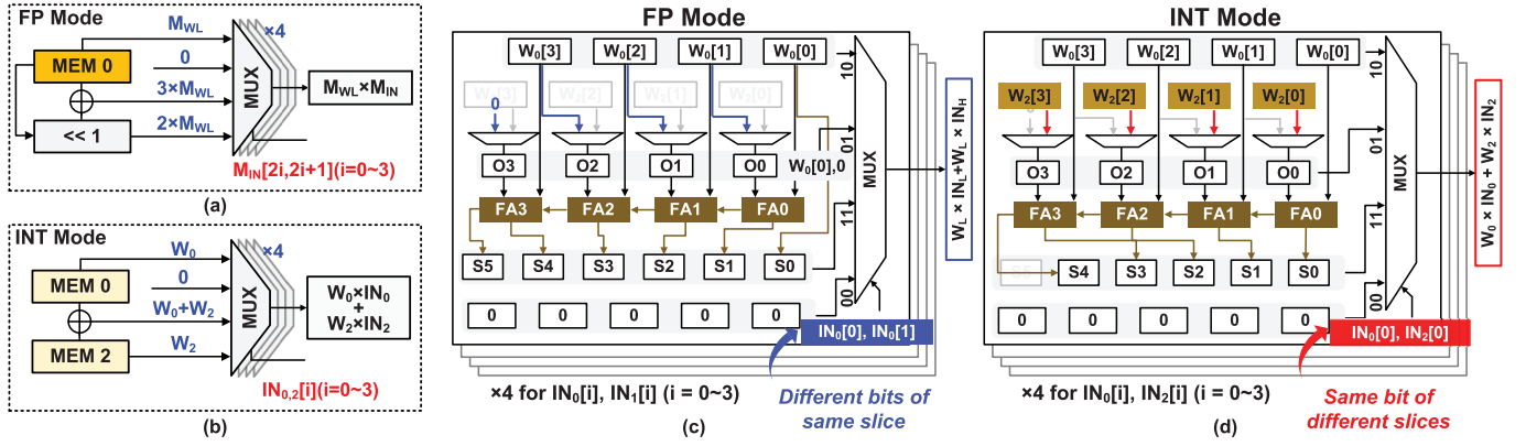
Fig. 7. FIC-LUT reconfigured as (a) FP-MAC and (b) INT-MAC operations. Detailed configurations of the FIC-LUT in (c) FP and (d) INT modes. With M_W = \{M_{WH}, M_{WL}\} = \{W_1, W_0\} and M_{IN} = \{IN_1, IN_0\} , the figure demonstrates FP-MAC operations using an INT format, highlighting the flexibility of the reconfigurable approach.
