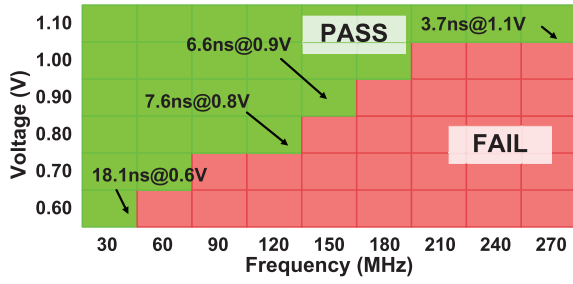
Fig. 16. Measured shmoo plot showing voltage versus working frequency.
