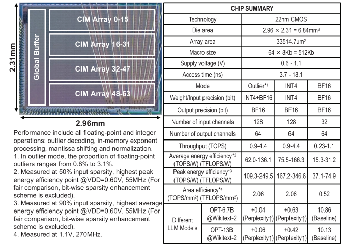
Fig. 15. Die photograph and chip performance summary.
