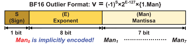
Fig. 6. Data format of BF16-outlier, highlighting the implicitly encoded leading one in the mantissa.
