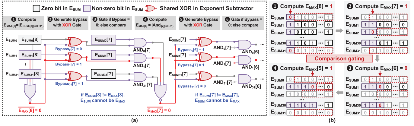
Fig. 9. (a) Construction of the bit-serial exponent comparator with the shared XOR logic. (b) Example of non-maximum exponent comparison gating.
