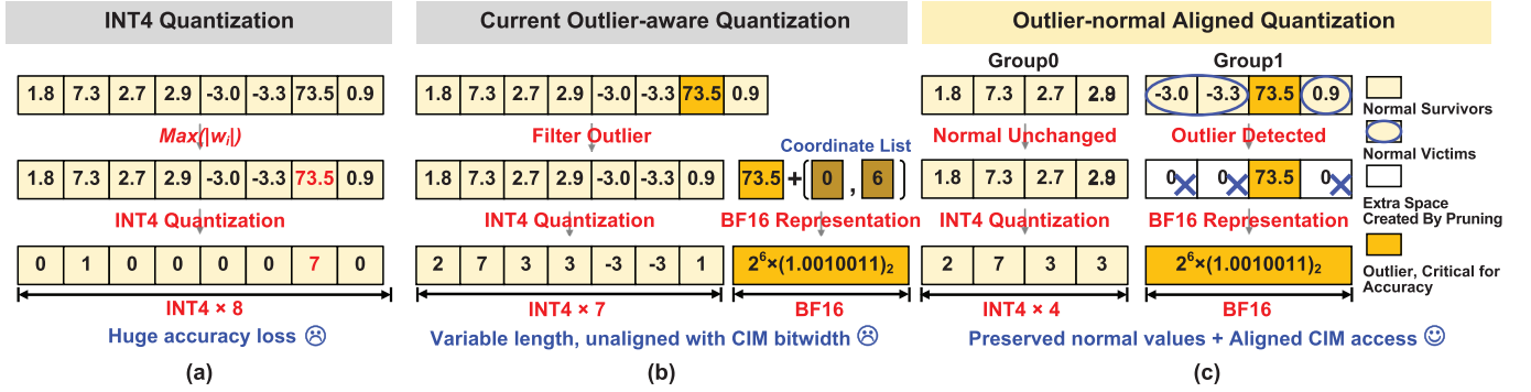
Fig. 3. Quantization methods comparison. (a) INT4 quantization. (b) Current OAQ. (c) Outlier-normal aligned quantization.
