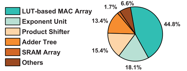
Fig. 19. Power breakdown of the proposed OA-CIM macro, obtained by post-layout simulation with Synopsys PrimeTime PX.
