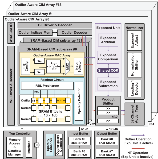
Fig. 4. Overall architecture of OA-CIM macro.
