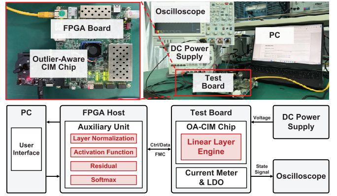
Fig. 14. Measurement setup of the OA-CIM chip.
